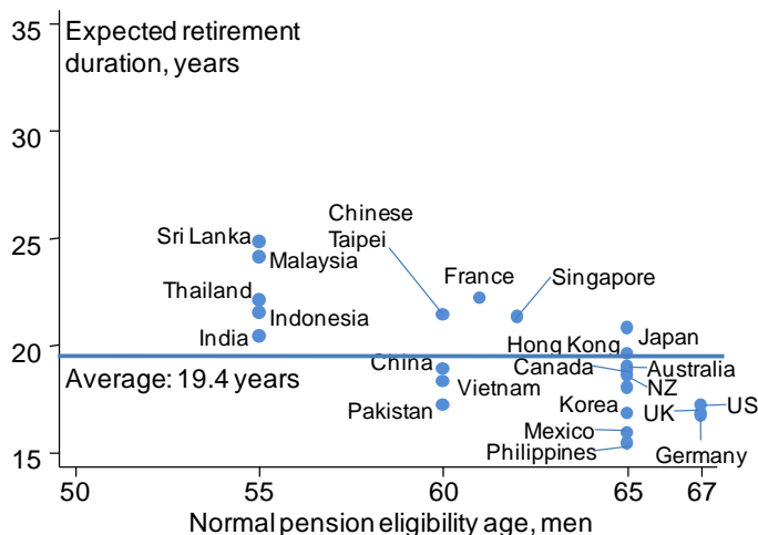
Figure 2. Expected time in retirement Men
