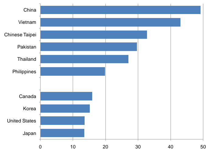
Figure 3. Required contribution rates
