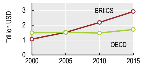
Cost of premature deaths from indoor air pollution (GDP equivalent, 2015)
