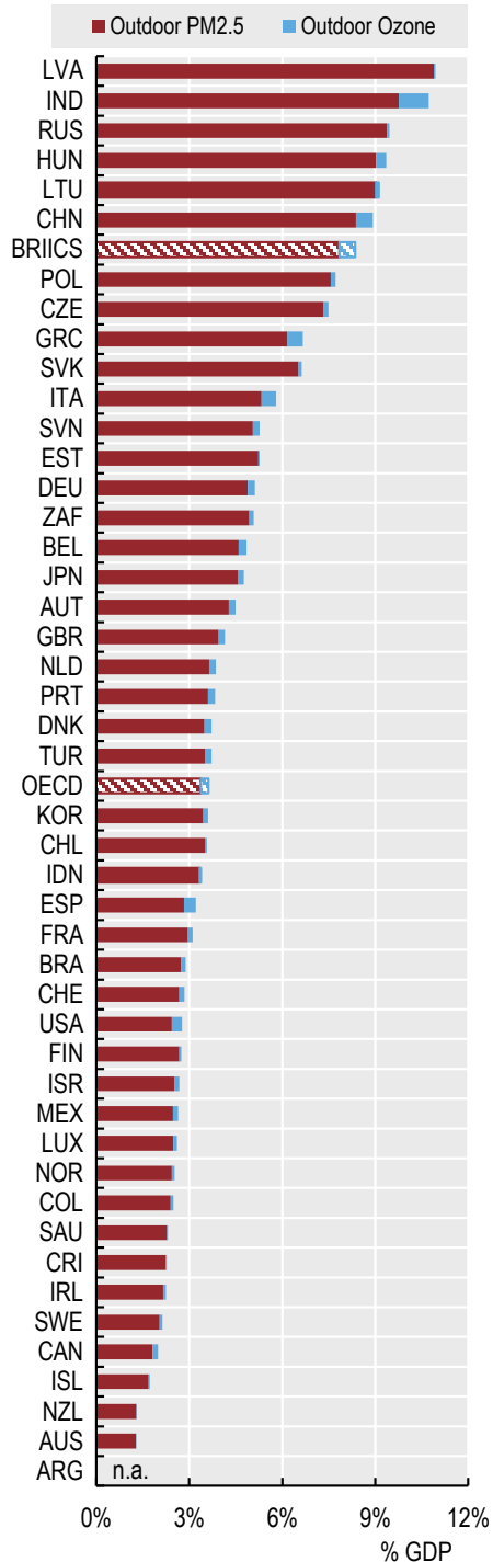
Cost of premature deaths from outdoor air pollution (GDP equivalent, 2015)
