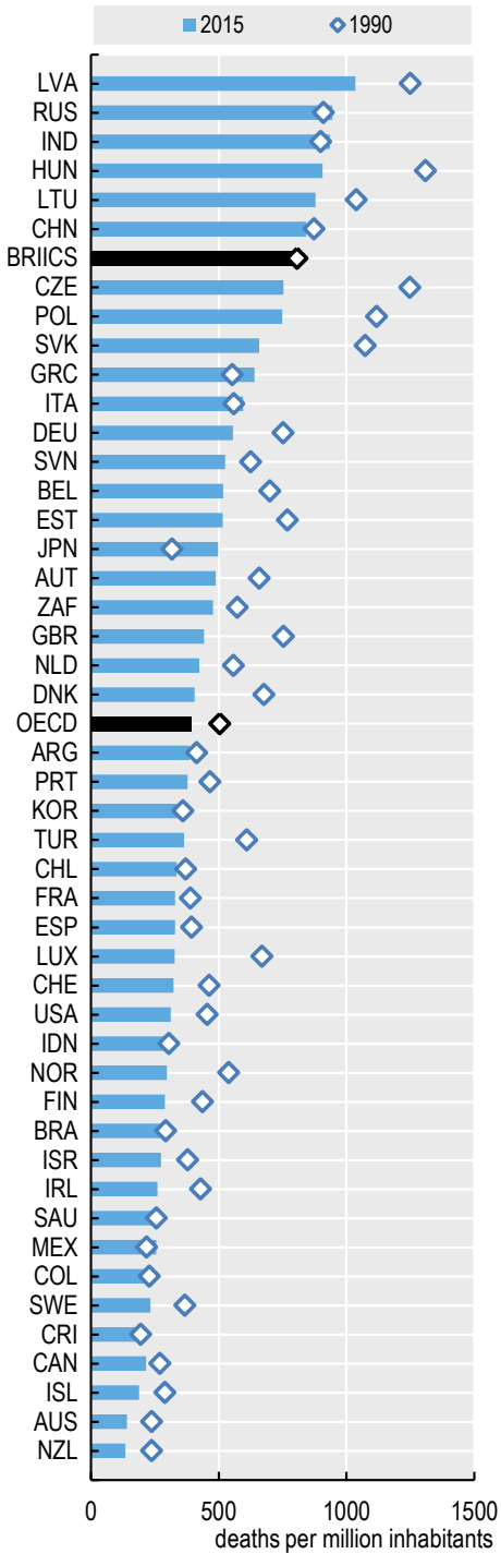
Mortality from outdoor air pollution (PM 2.5 and O 3 )
