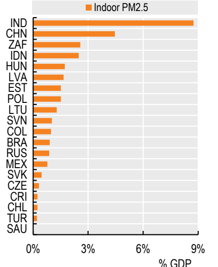
Mortality from indoor air pollution
