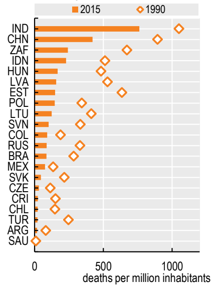
Mortality from indoor air pollution
