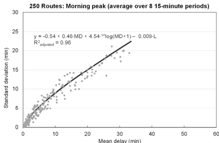
Figure 3.8. Mean delay versus standard deviation fitted with a combination of a linear and a logarithmic function
