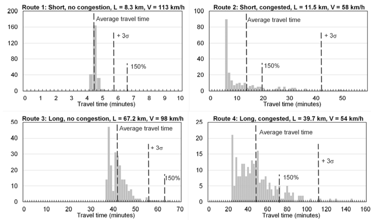
Figure 3.2. Travel-time distributions for four routes with different characteristics
