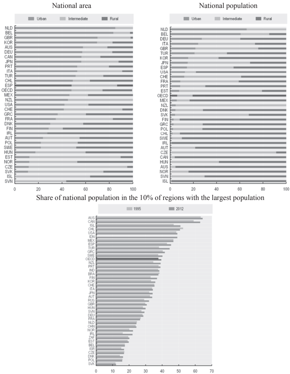
Figure 4.2. Distribution of the national area and national population into urban, intermediate and rural regions (top) and share of national population in the 10% of regions with the largest population (bottom)
