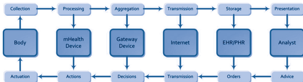
Figure 9.2. mHealth pipeline
