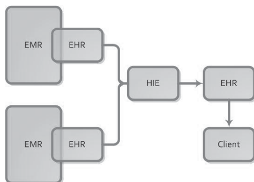
Figure 9.1. HIE architectures
