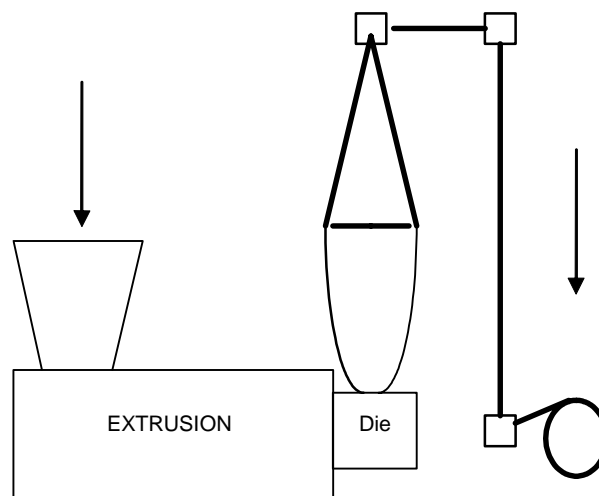
Film extrusion
