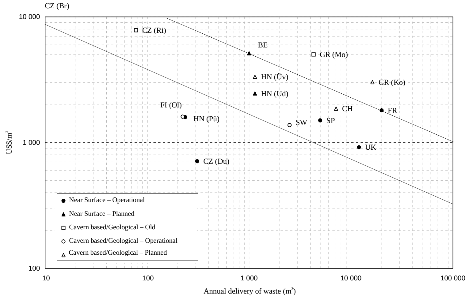
Figure 4.2.3 (c) Operating costs versus annual delivery
