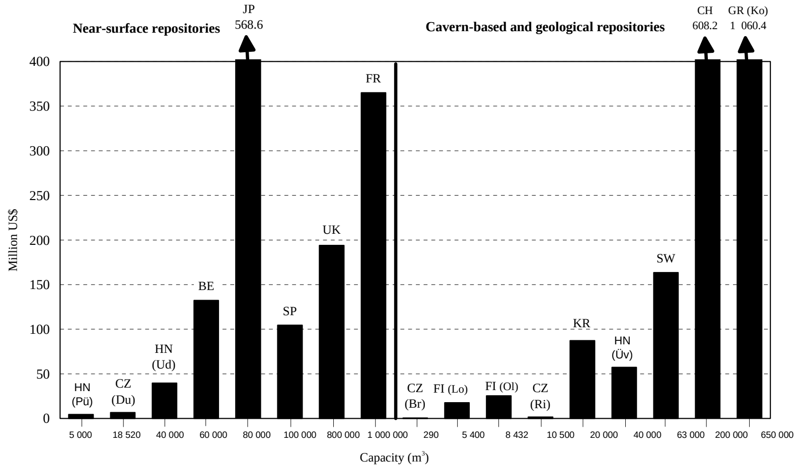
Figure 4.2.2 (a) Construction costs versus capacity
