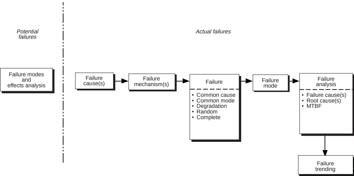
Figure 7. Examples of causes, mechanism, and modes
