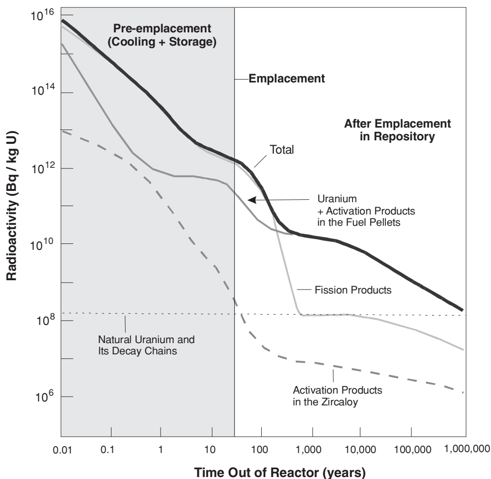
Figure 2.1: An example of the decrease of the activity of Canadian spent fuel over time due to radioactive decay (from the Atomic Energy of Canada Limited 1994 Environmental Impact Statement, AECL, 1994)
