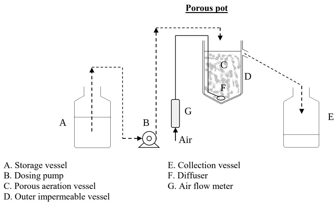
Figure 2: Equipment used for assessment of biodegradability
