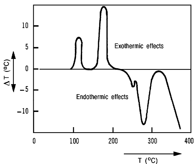
Figure 2: DTA curve
