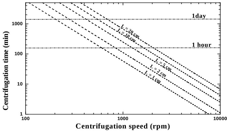
Fig. 1b Variations of centrifugation time ( t ) versus centrifugation speed (rpm) for different lengths of the mixture in the centrifuge tube (R_b - R_t) = L ; R_t = 10\text{ cm} , \eta = 8.95 \times 10^{-3}\text{ g s}^{-1}\text{ cm}^{-1} , \rho_{aq} = 1.0\text{ g cm}^{-3} at 25^\circ\text{C} and \rho_s = 2.0\text{ g cm}^{-3} .
