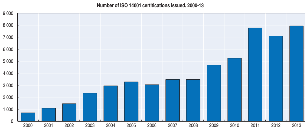
Figure 2.3. A sharp increase in the number of ISO 14001 EMS certificates
