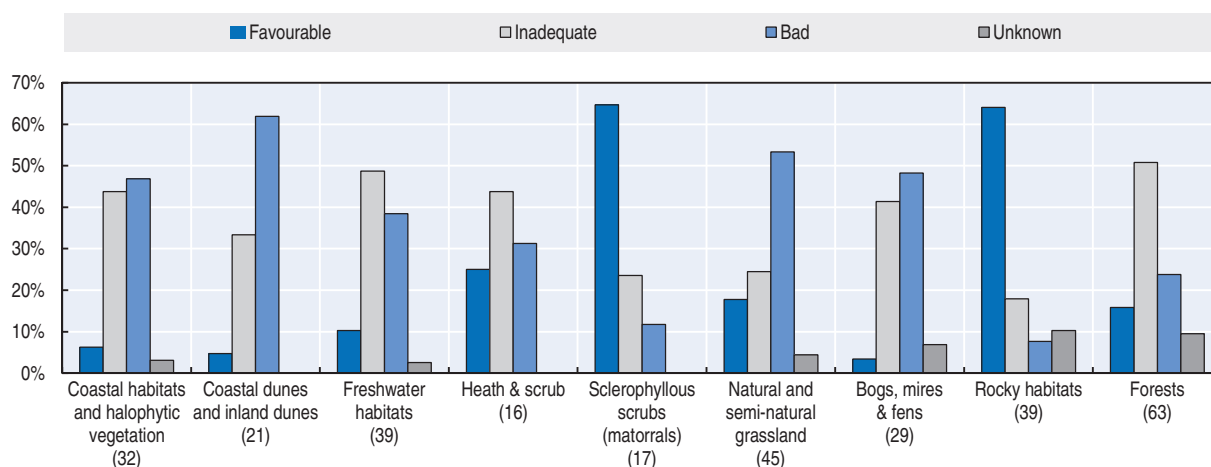
Figure 5.1. Three-quarters of habitats of Community interest have an unfavourable conservation status
