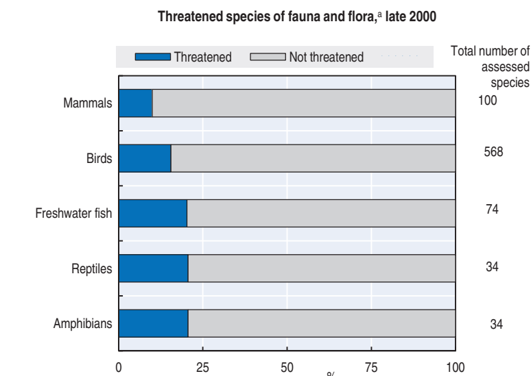
Figure 1.18. In metropolitan France, one species in five is threatened
