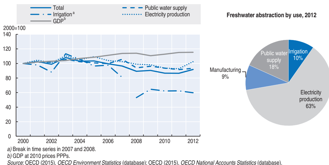
Figure 1.19. Water abstraction is declining
