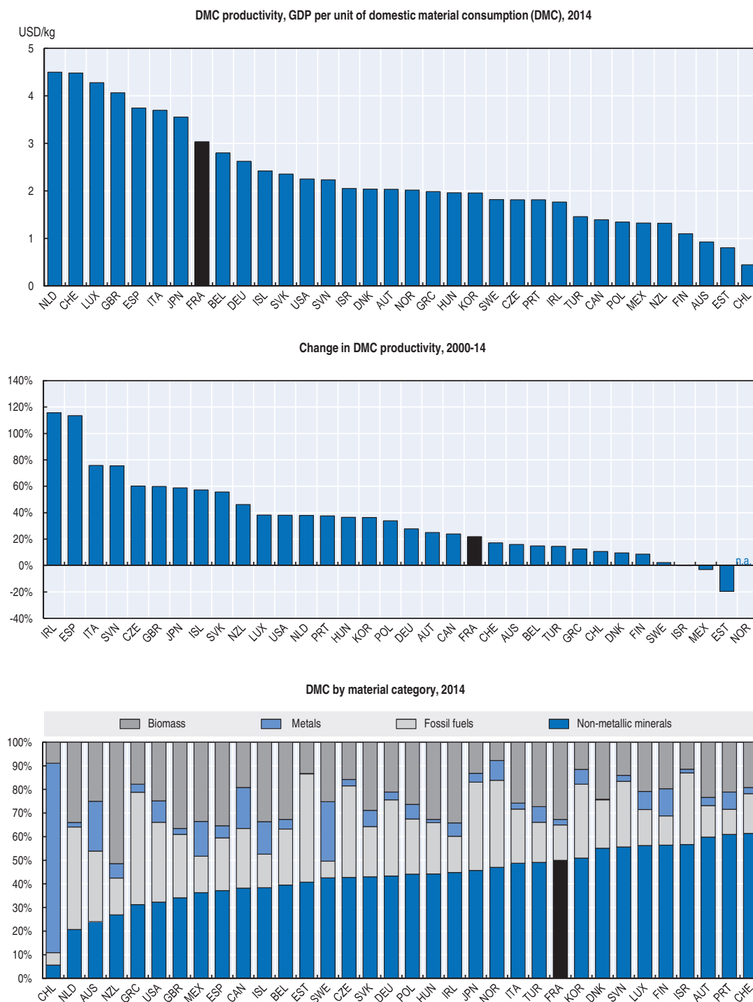
Figure 1.C2. Material consumption and resource productivity
