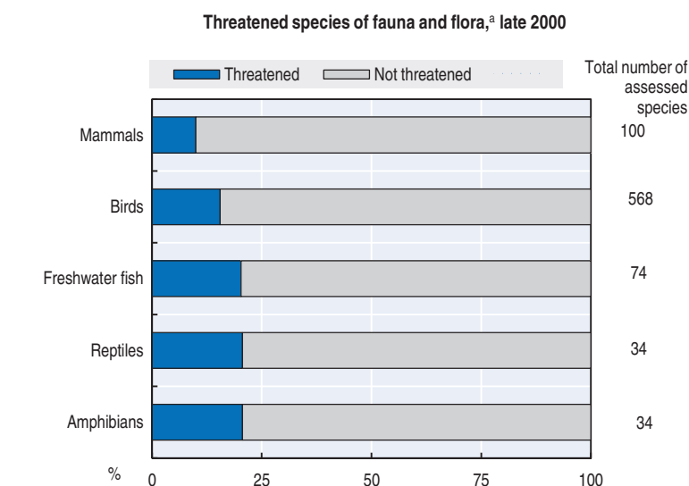
Figure 5.3. One out of five species is threatened in metropolitan France
