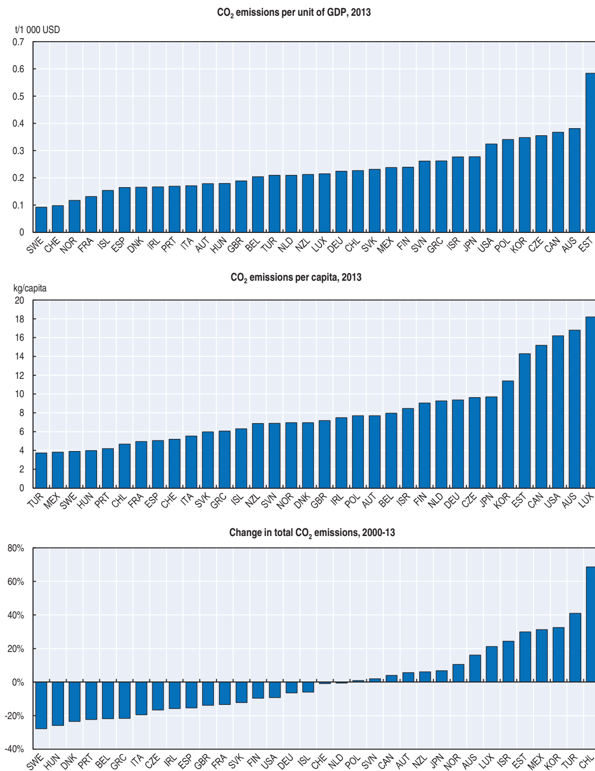
Figure 1.B2. CO 2 emissions and intensities
