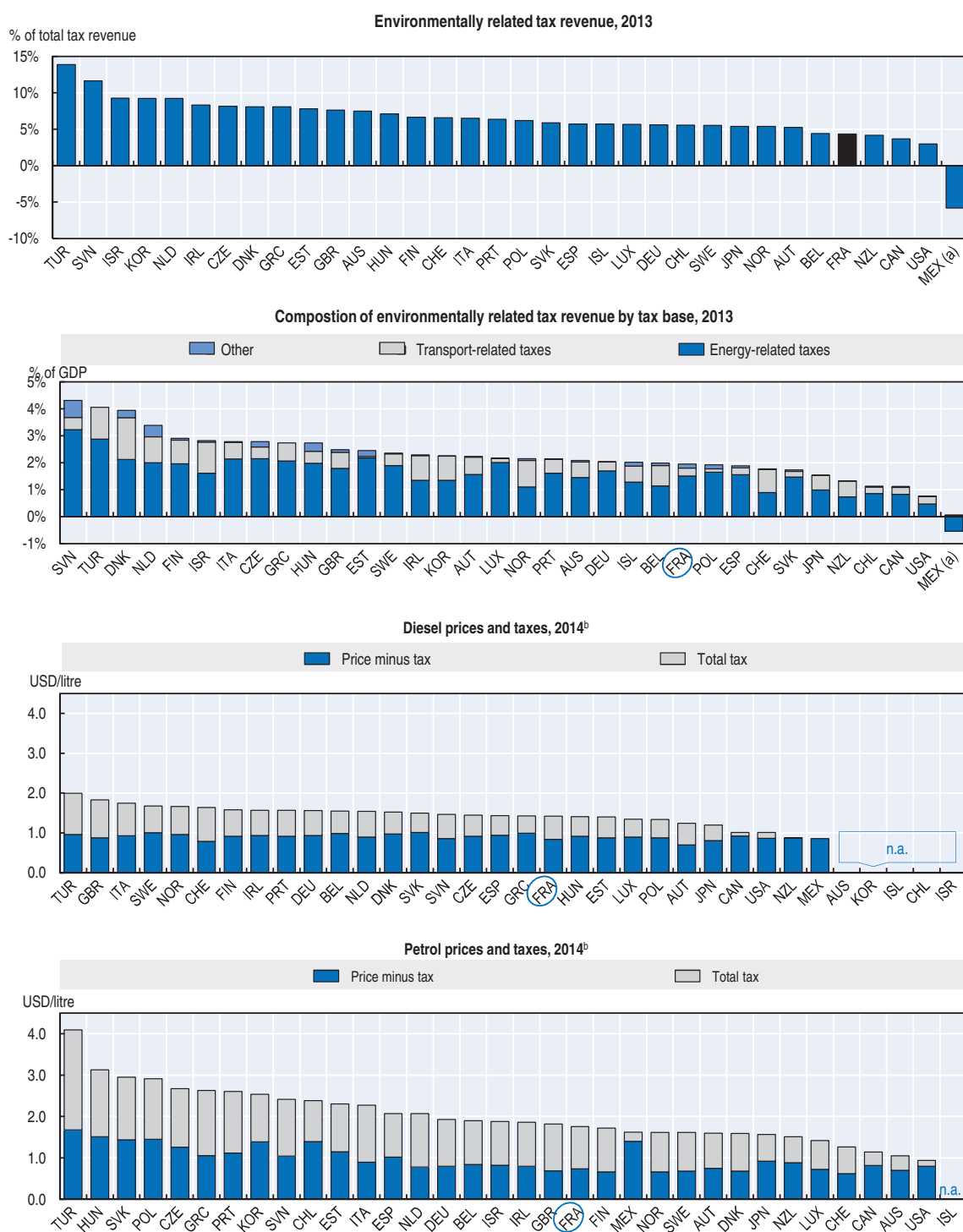
Figure 3.A1. Environmentally related taxes
