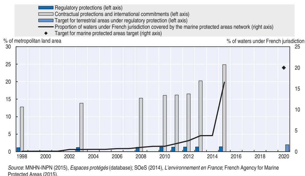
Figure 1.16. Protected areas are expanding in metropolitan France
