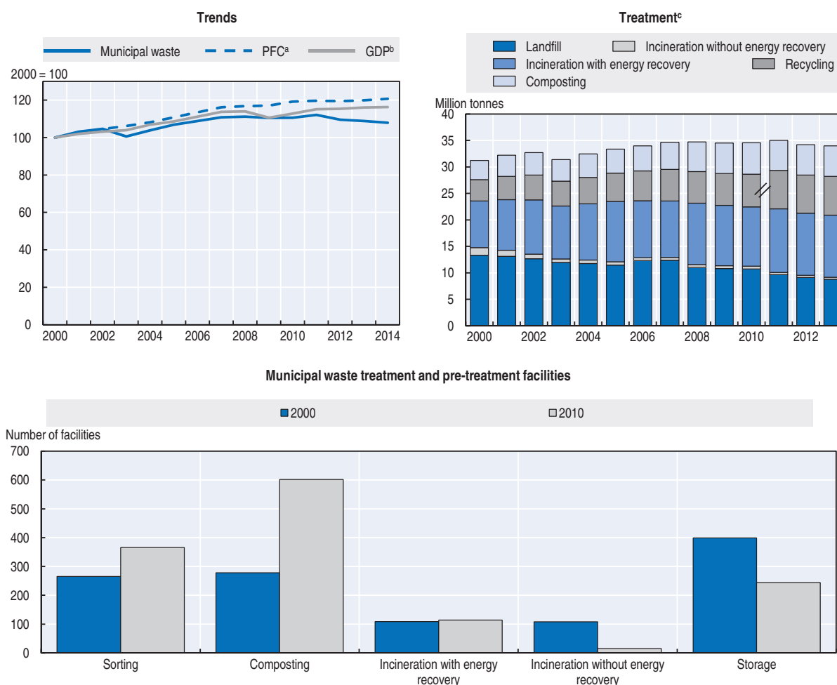
Figure 1.13. Municipal waste production is slowing, while waste recovery is progressing slowly
