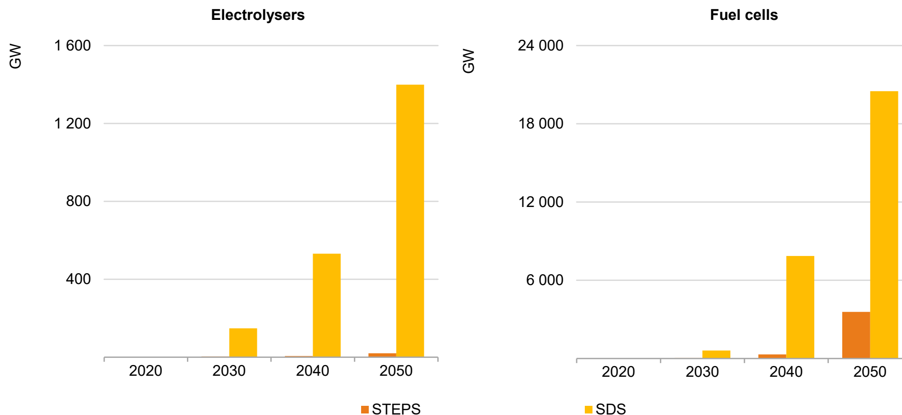
Global installed capacity of electrolysers and fuel cells in the SDS
