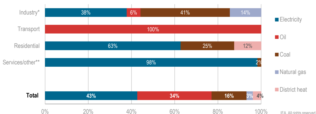
Figure 2.8 Total final consumption by source and sector, 2020
