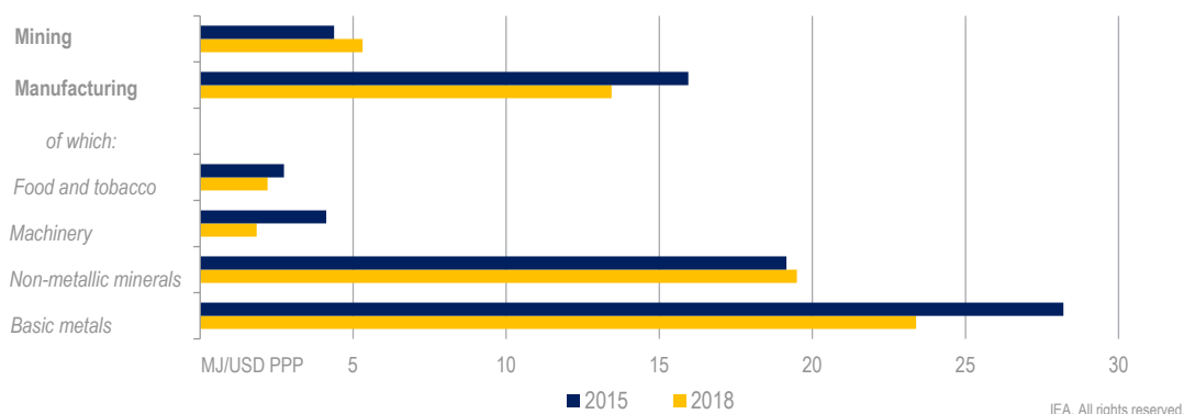
Figure 8.8 Selected intensities in the industrial sector
