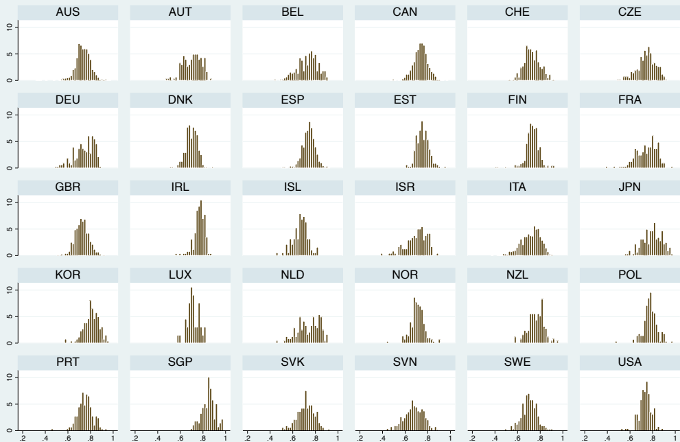
DEA efficiency scores
