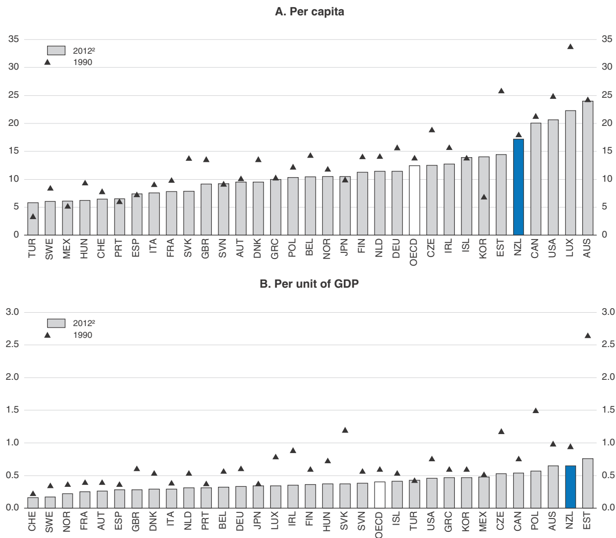
Figure 12. GHG emissions per capita and per unit of GDP
