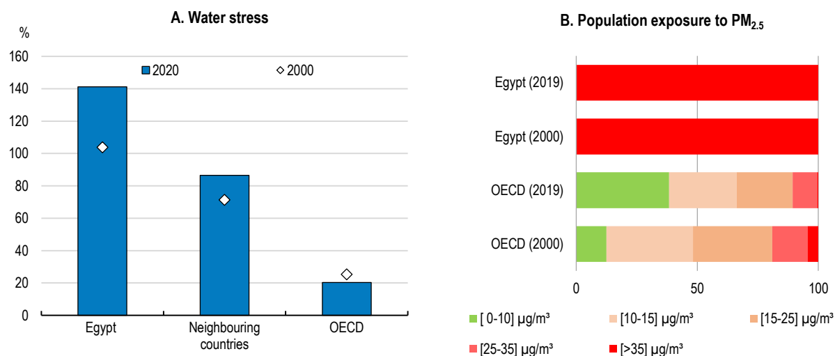
Figure 1.8. Further efforts to reduce emissions are needed
