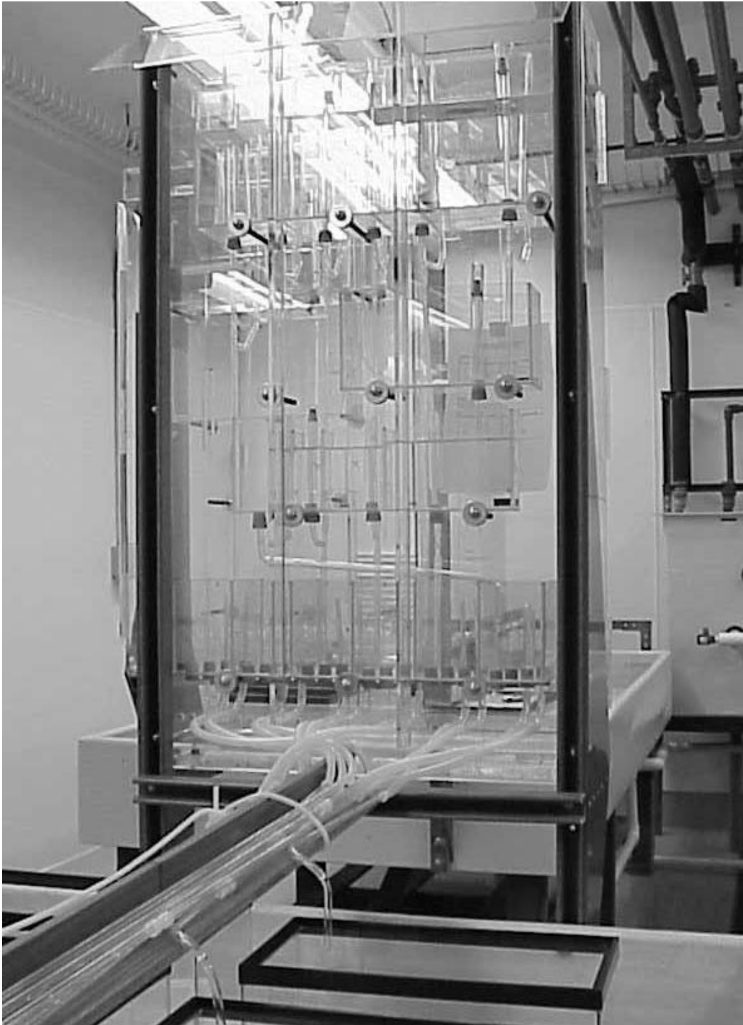
Figure 1. Diluter
