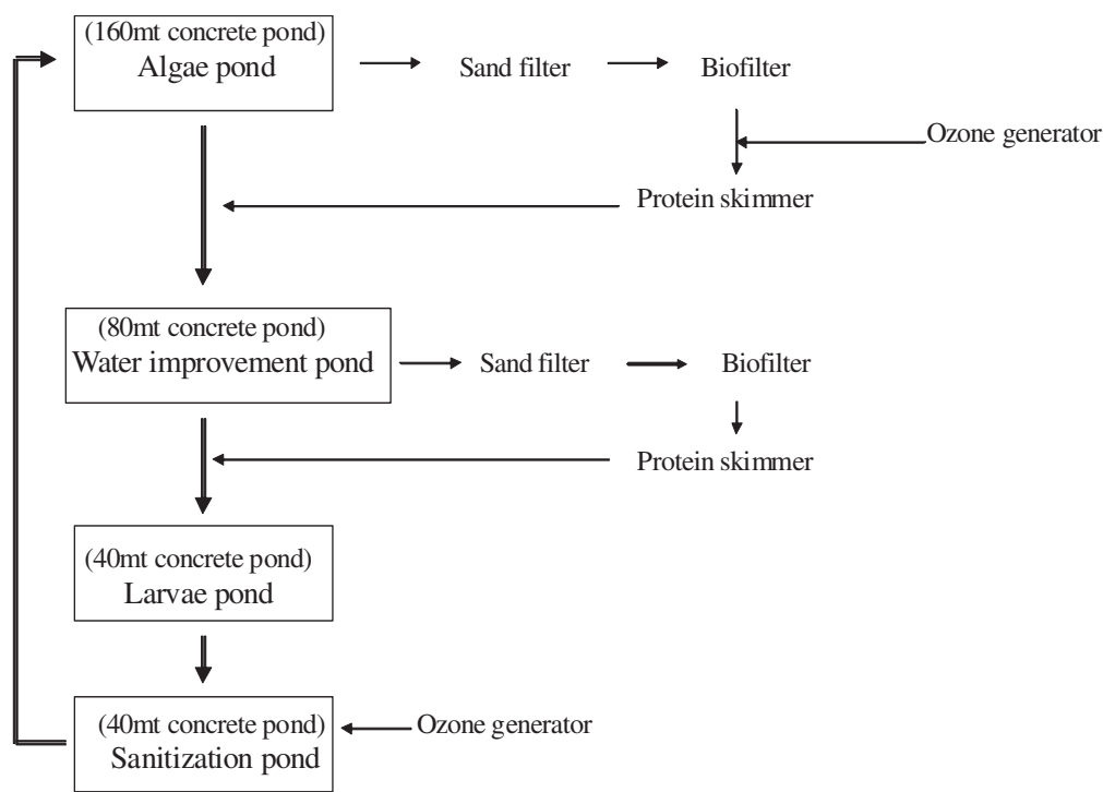
Figure 12.1: Green water recirculation system for larviculture
