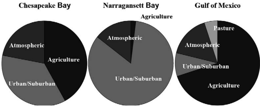
Figure 14.1: Comparison on the relative distribution of majour souces of nitrogen pollution in three coastal eco-systems experiencesing hypoxia
