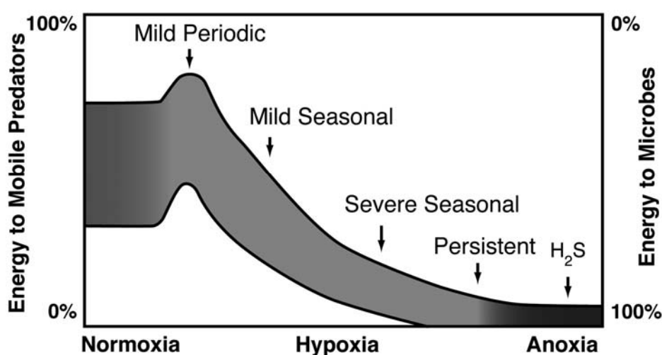
Figure 14.5: Conceptual view of how hypoxia alters ecosystem energy flow
