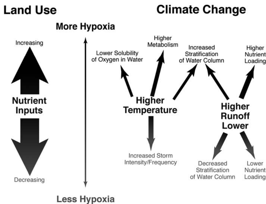
Figure 14.7: Relative contribution of global climate change and land use to future hypoxia
