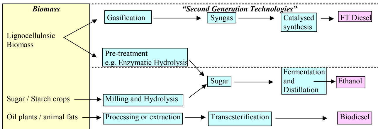
Figure 1. Fuel production pathways
