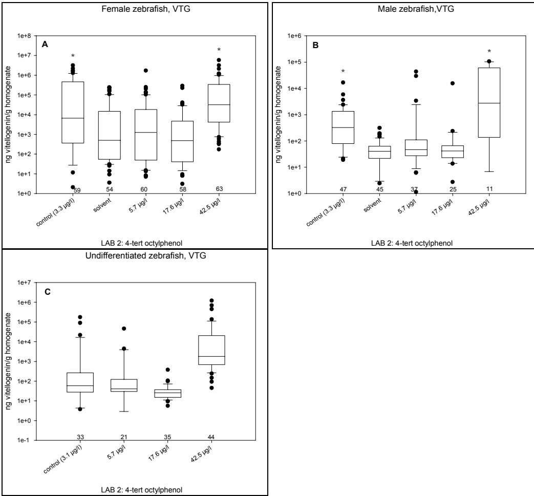
Figure 4: Vitellogenin concentrations in female (A), male (B) and undifferentiated (C) zebrafish after 60 D exposure to 4-tert-octylphenol. Numbers at the bottom are N. P=0.05. *=Significant different from control
