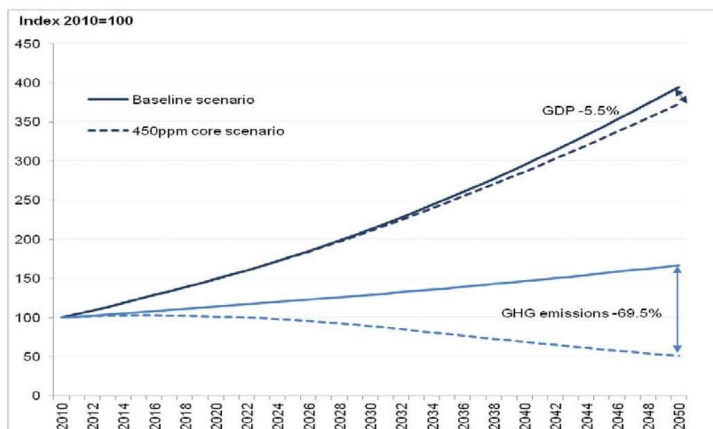
Figure 1.2. Global emissions and cost of mitigation
