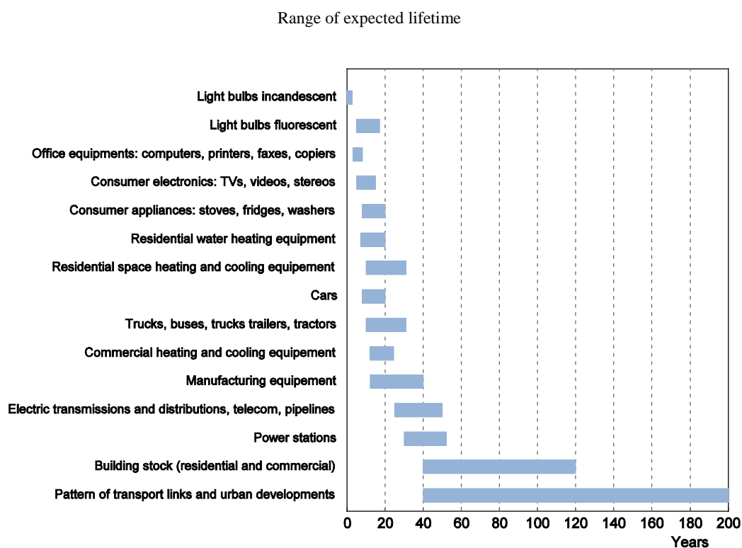
Figure 3.1. Capital stock turnover times for selected energy-related stock
