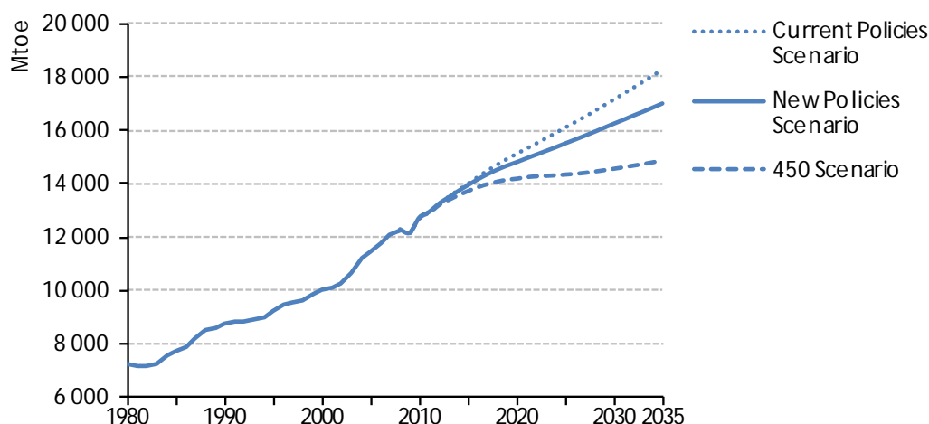
Figure 1.3. World primary energy demand by scenario
