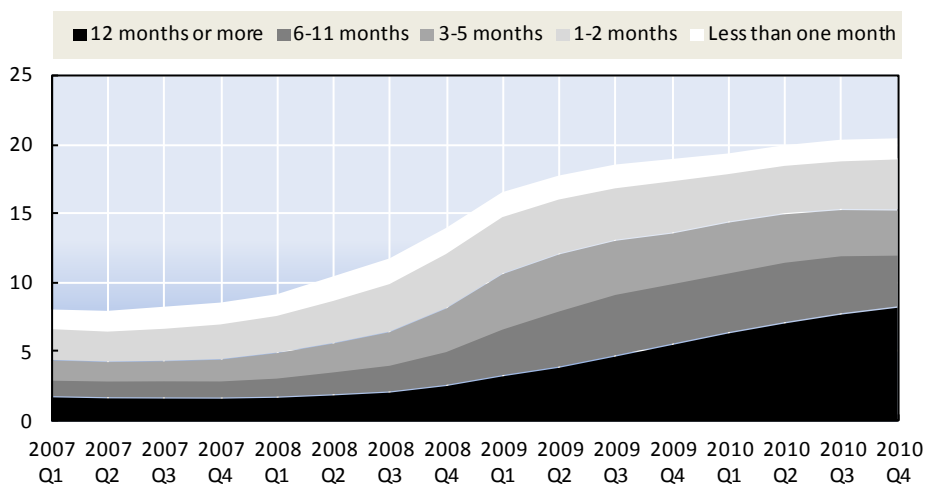
Evolution of unemployment by duration of unemployment (percentage of the labour force), Spain
