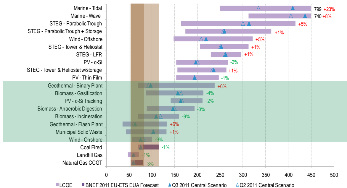
Figure 1: Levelised cost of energy q3 2011 ($/mWH)
