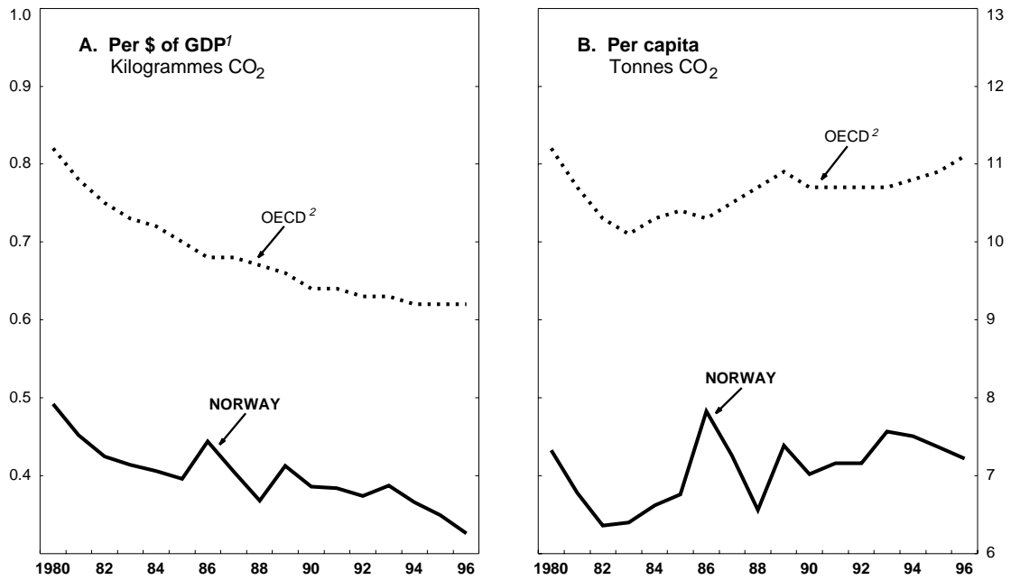
Figure 4. Carbon dioxide emissions
