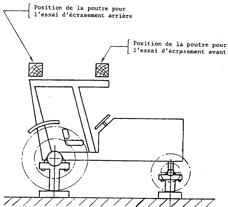
Figure 4.7.a Cabines de protection
