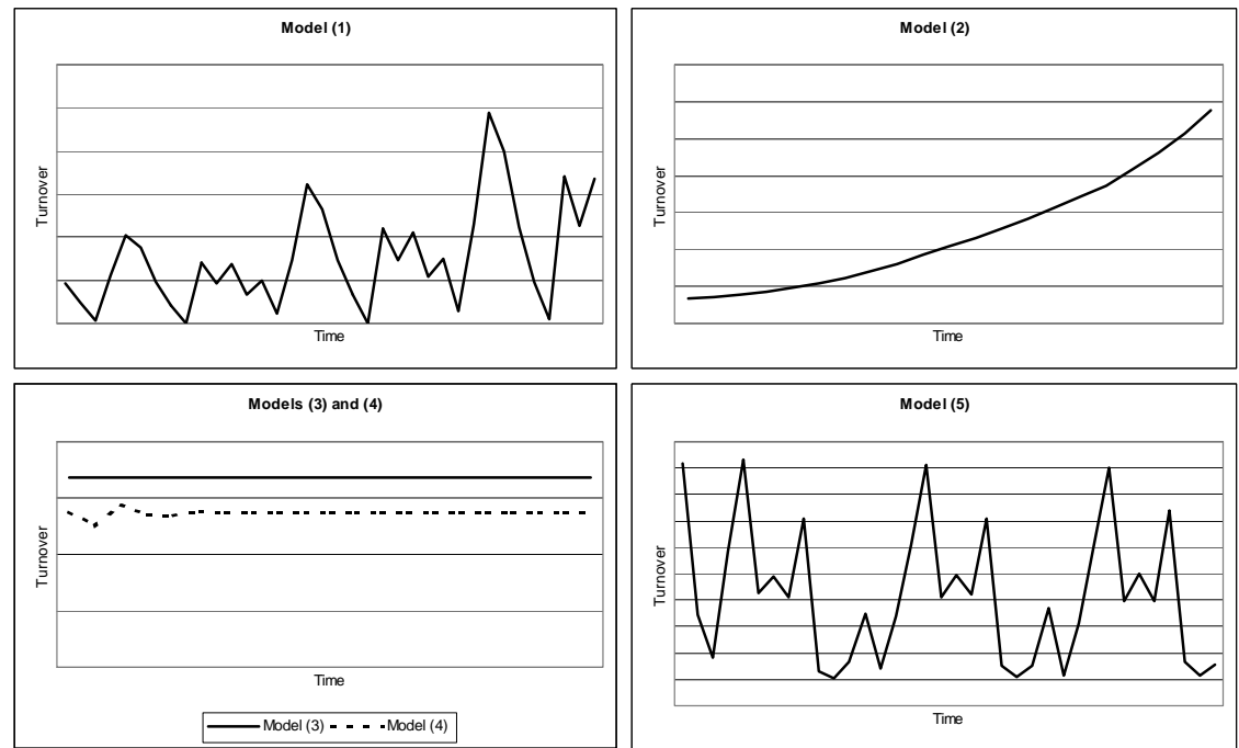
Picture 5: Illustration of the imputation methods
