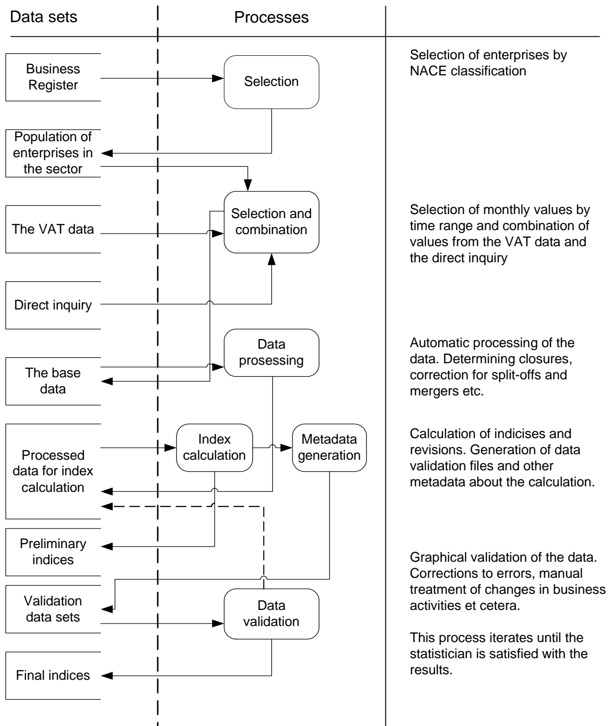
Picture 1: The compilation process
