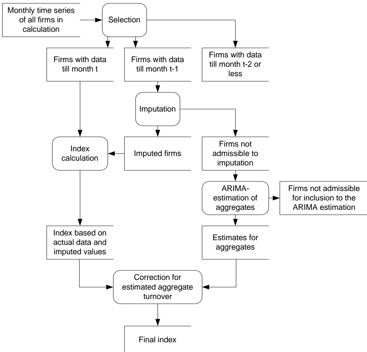
Picture 3: Overview of the imputation and estimation methods
