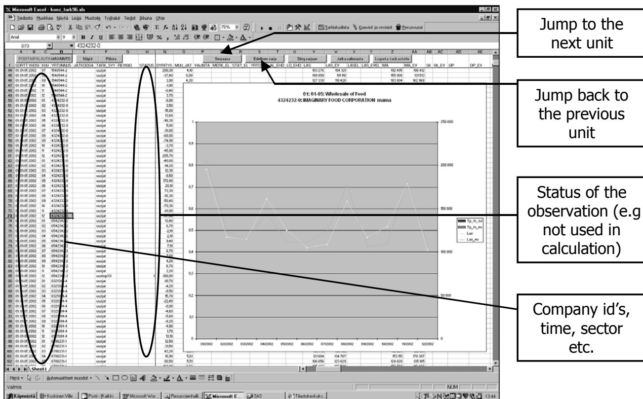
Picture 2: Graphical data validation
