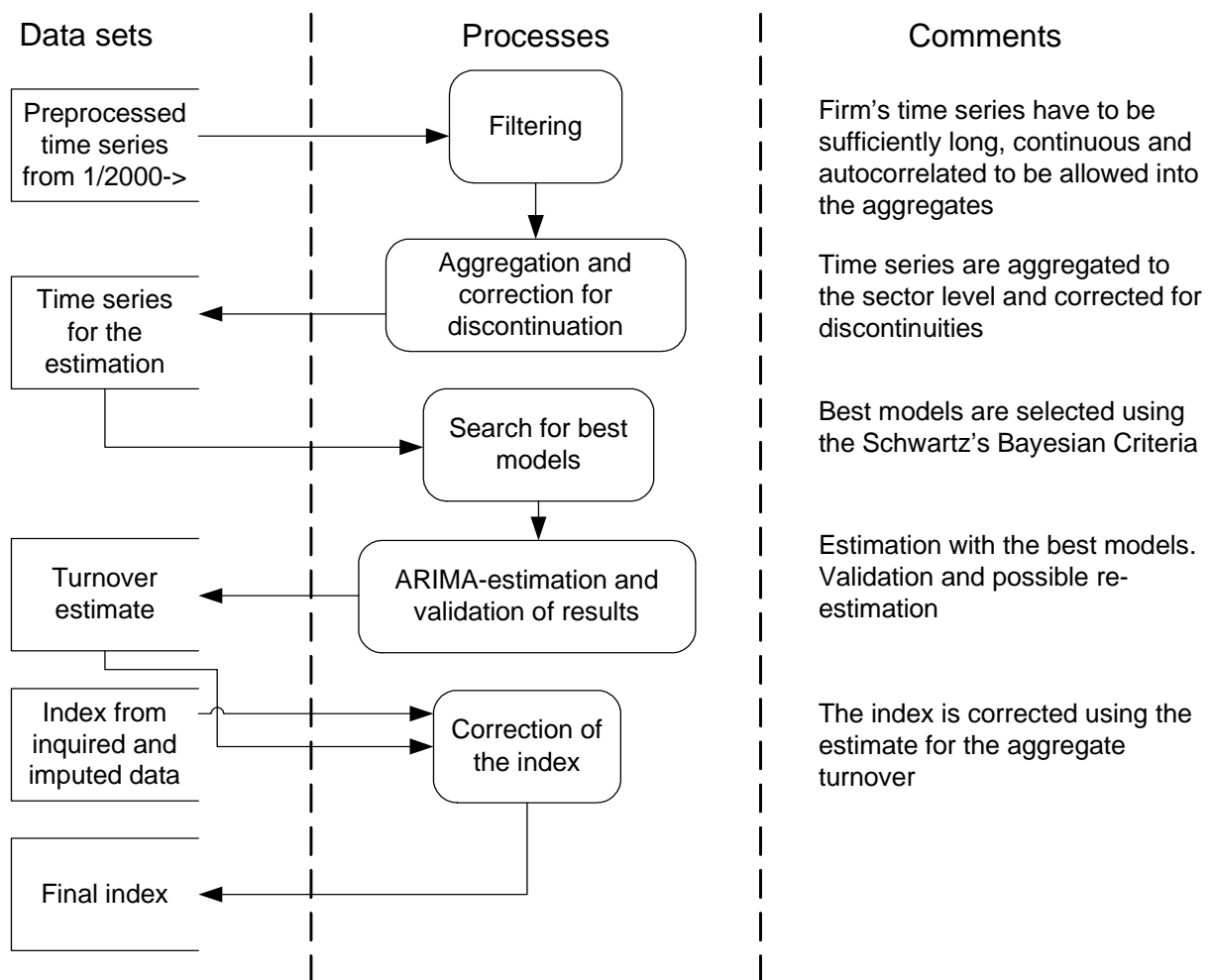
Picture 6: The ARIMA-estimation process
