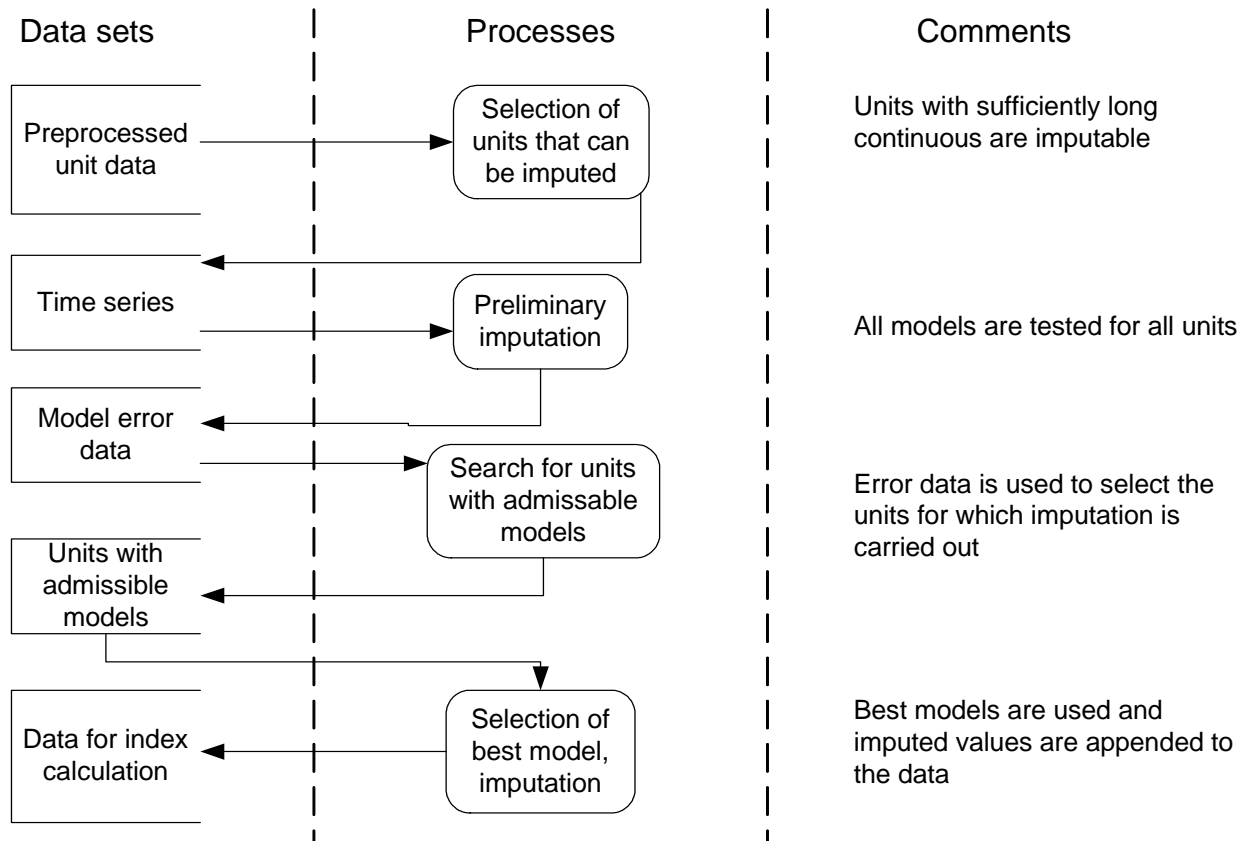
Picture 4: The imputation process
