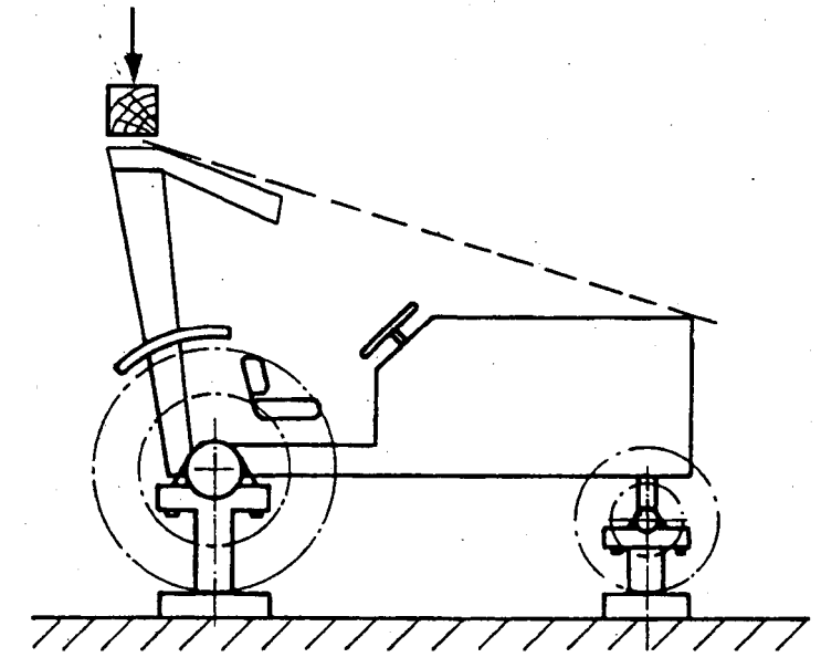
Figure 3.10(b): Rear roll bar frame
