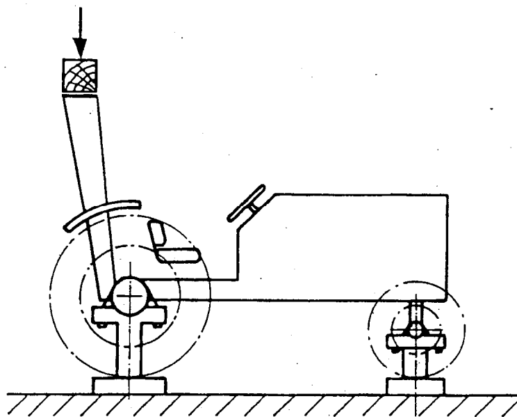
Figure 3.9(b): Rear roll bar frame
