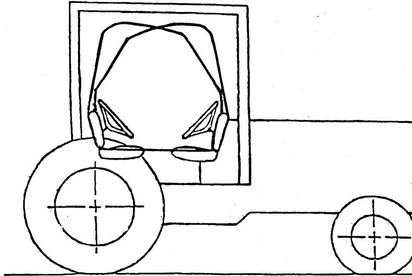
Figure 3.14(a): Protective cab
