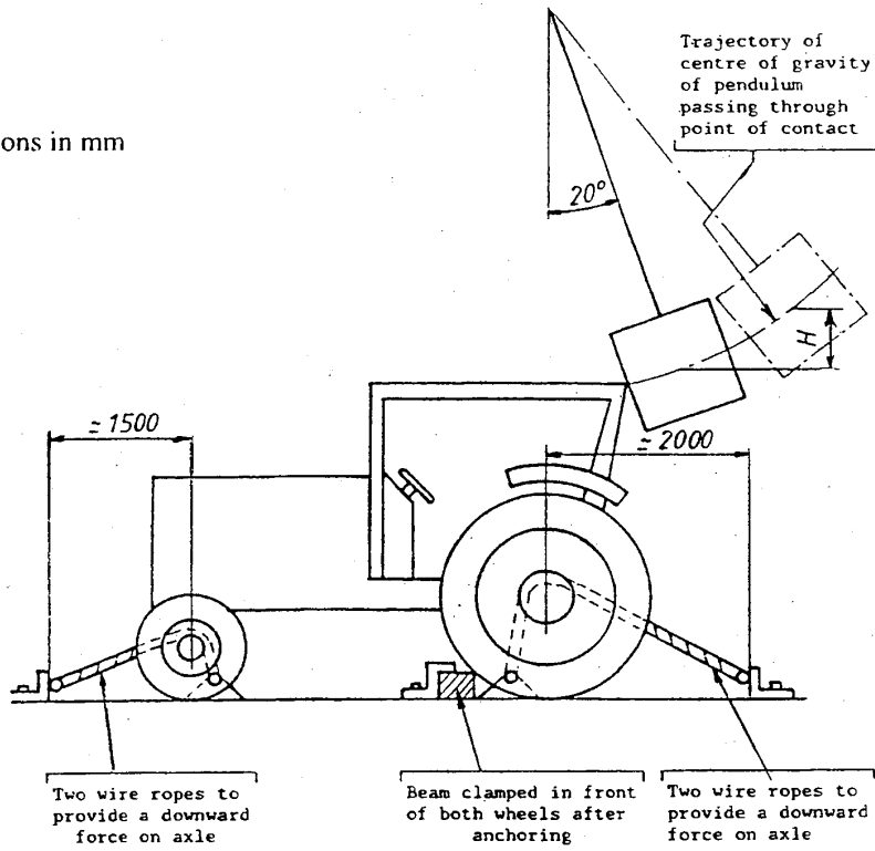
Figure 3.5(a): Protective cab
