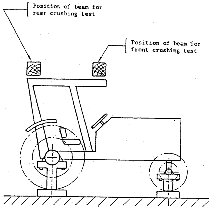
Figure 3.9(a): Protective cab
