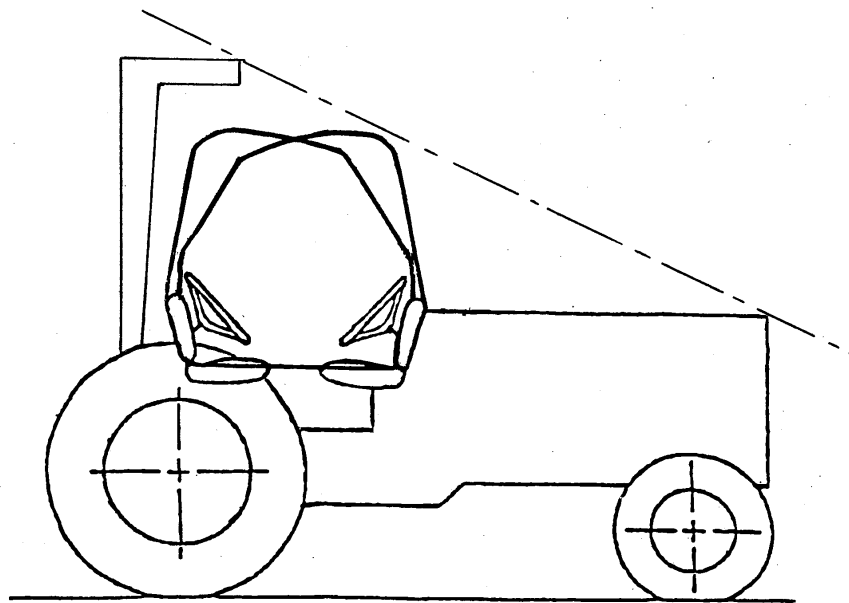
Figure 3.14(b): Rear roll bar frame
