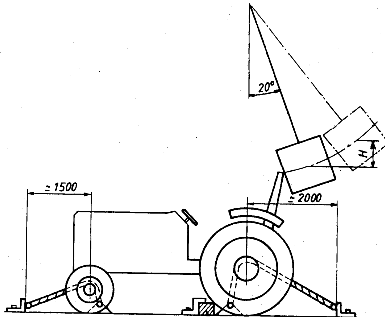
Figure 3.5(b): Rear roll bar frame Method of impact from rear for protective cab and rear roll bar frame
