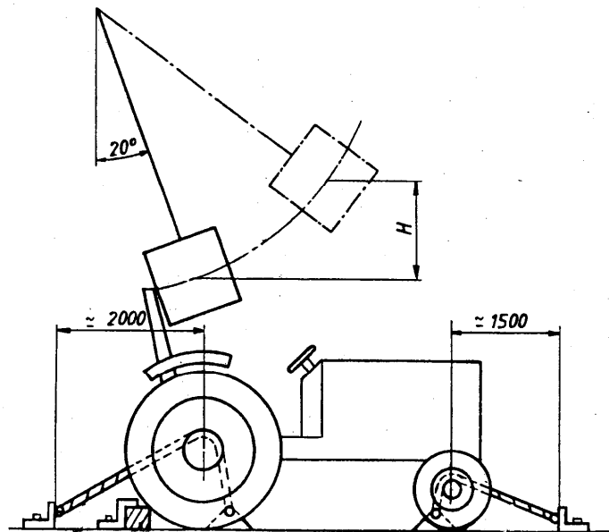
Figure 3.6(b): Rear roll bar frame
