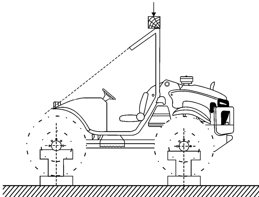
Figure 9.14 Rear roll bar frame
