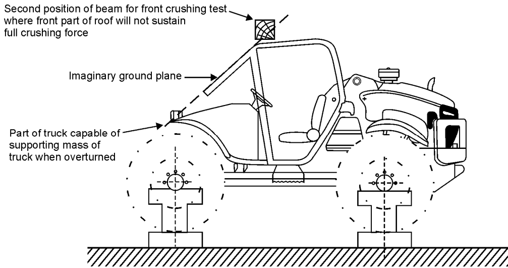
Figure 9.13 Protective cab
