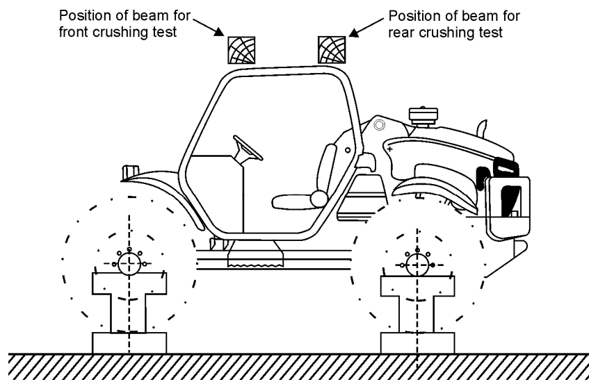
Figure 9.11 Protective cab
