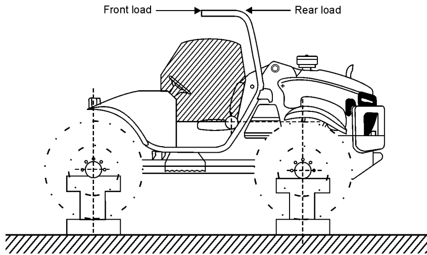
Figure 9.5 Rear roll bar frame
