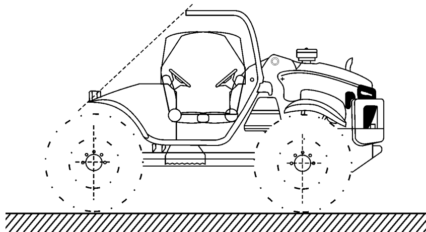
Figure 9.19 Rear roll bar frame
