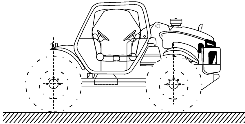
Figure 9.18 Protective cab
