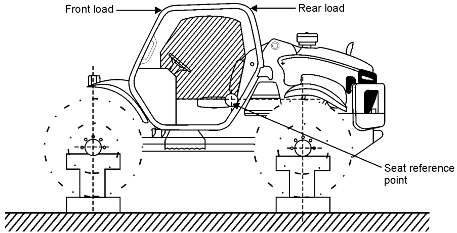
Figure 9.4 Protective cab
