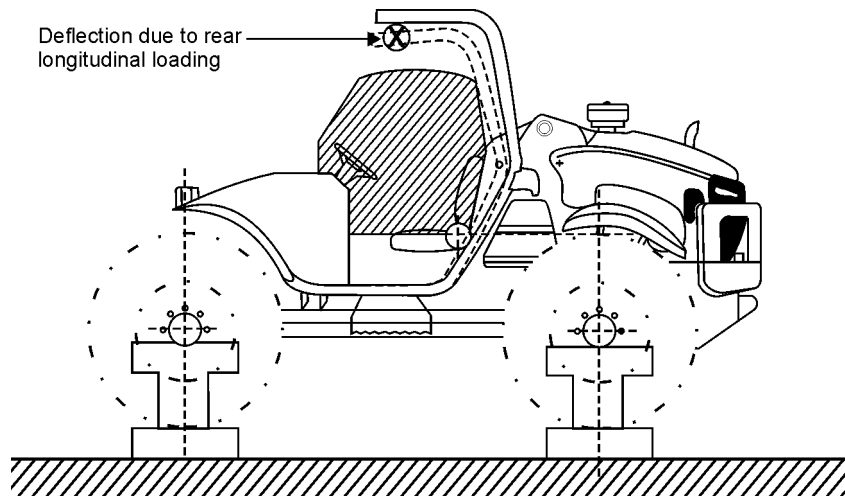
Figure 9.8 Rear roll bar frame
