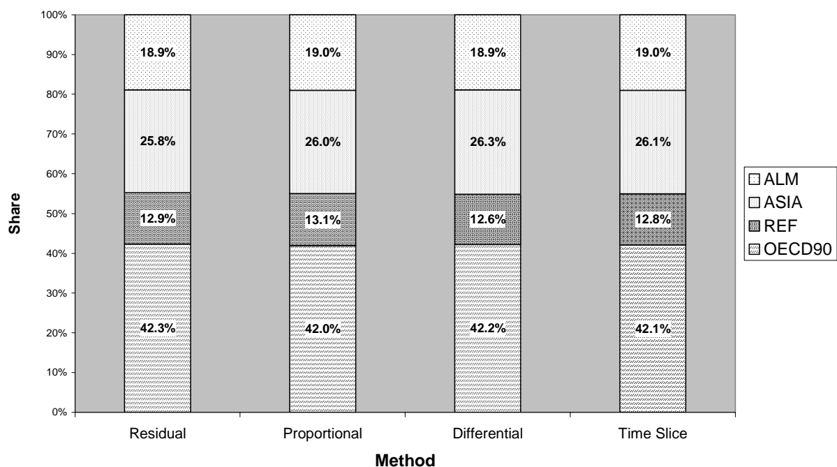
Figure 6. Illustrative results from CSIRO of the attribution calculation for temperature change in 1990 using different attribution methods. Includes emissions of CO 2 , CH 4 and N 2 O between 1890 and 1990 as provided in EDGAR-HYDE 1.3; earlier emissions were linearly extrapolated
