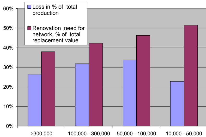
Figure 5.4 Losses in water production
