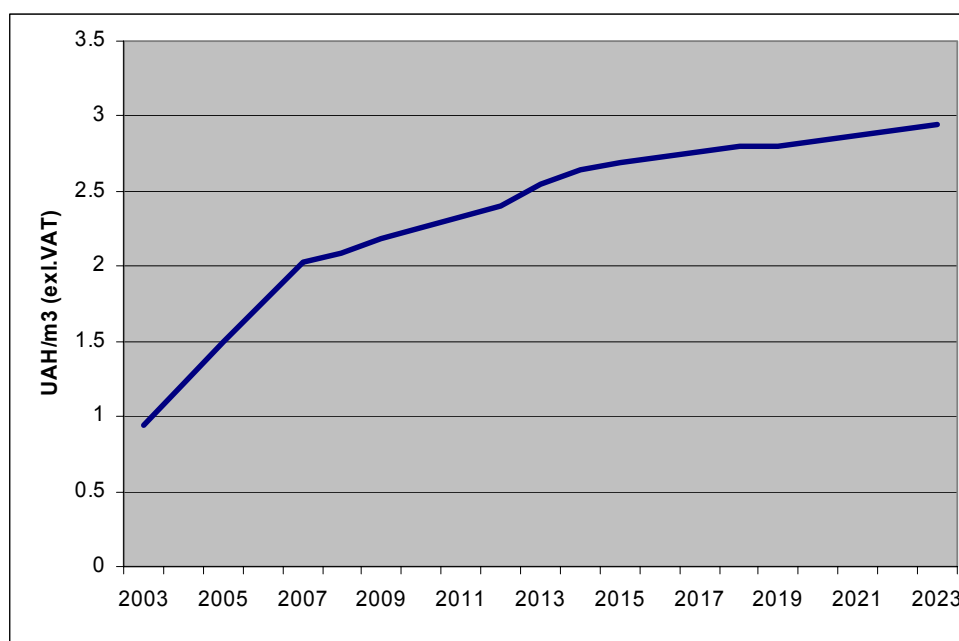
Figure 6.2 Non-household tariff profile at full O&M cost recovery
