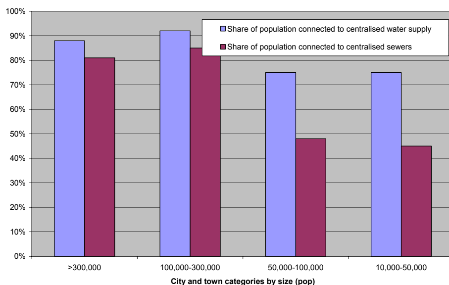
Figure 2.2 Water supply and wastewater connectivity
