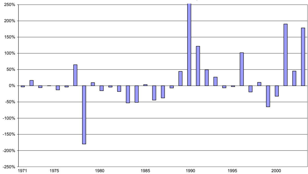
Figure 3. Relative differences bewtween GL (or KB) cost- and profit-based measures of TFP All industries in the Italian economy
