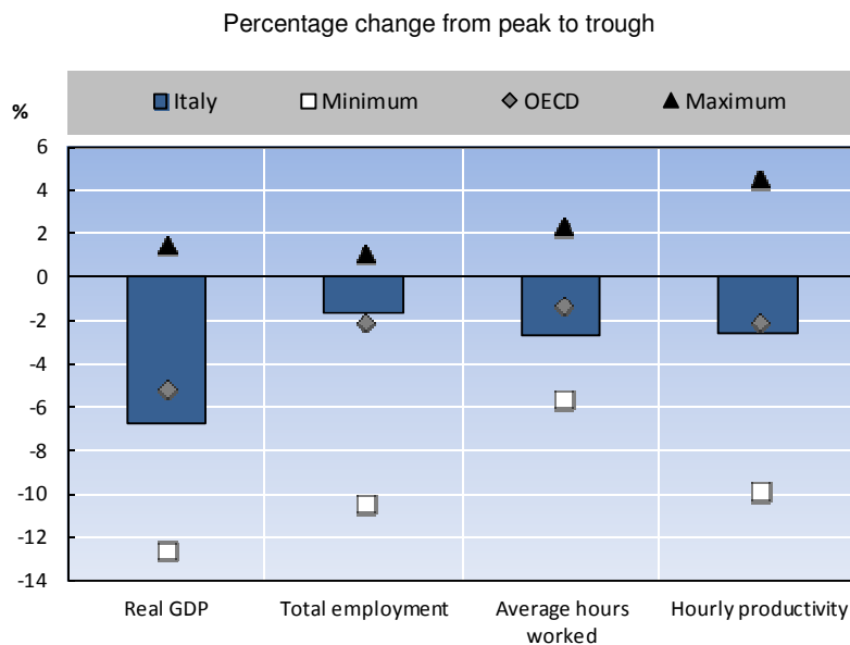
Figure 1. The impacts of the recession on employment, hours and productivity differed strikingly across countries
