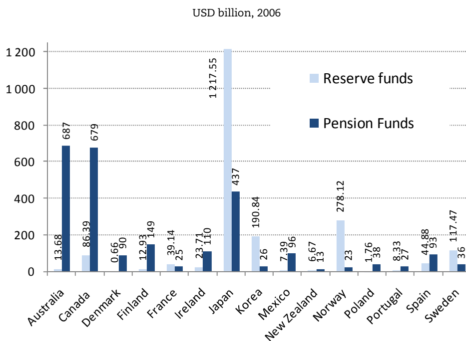
Figure 1. Reserve funds and pension funds in selected OECD countries
