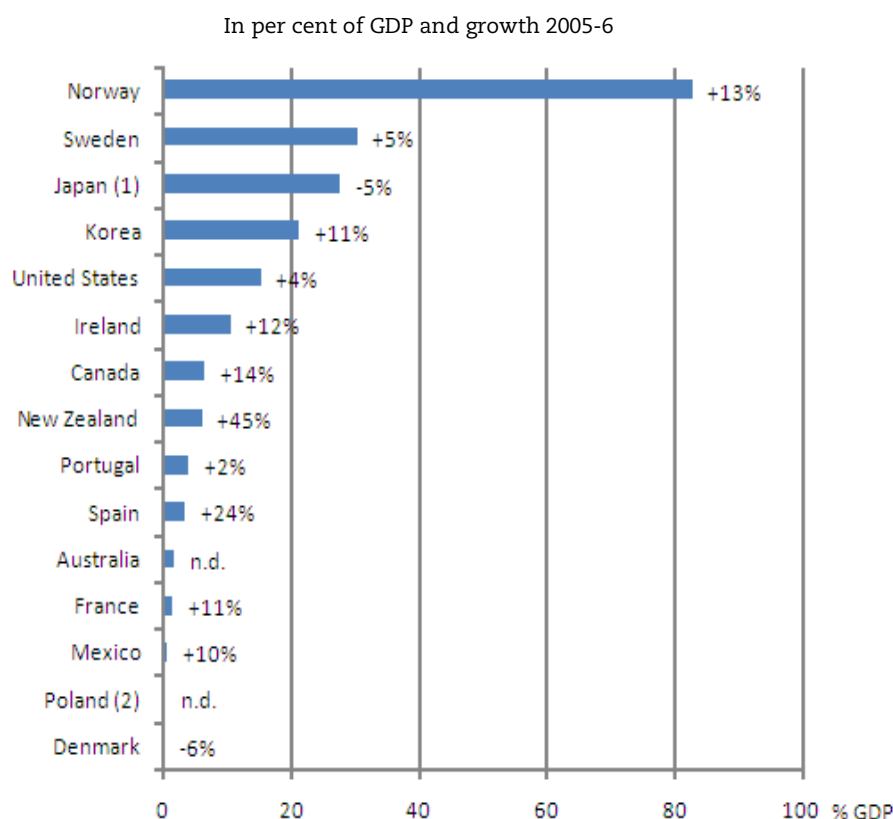
Figure 2. Assets accumulated in reserve funds
